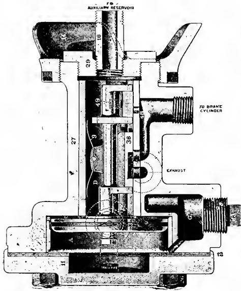
Fig. 1750. Plain Triple-valve.
